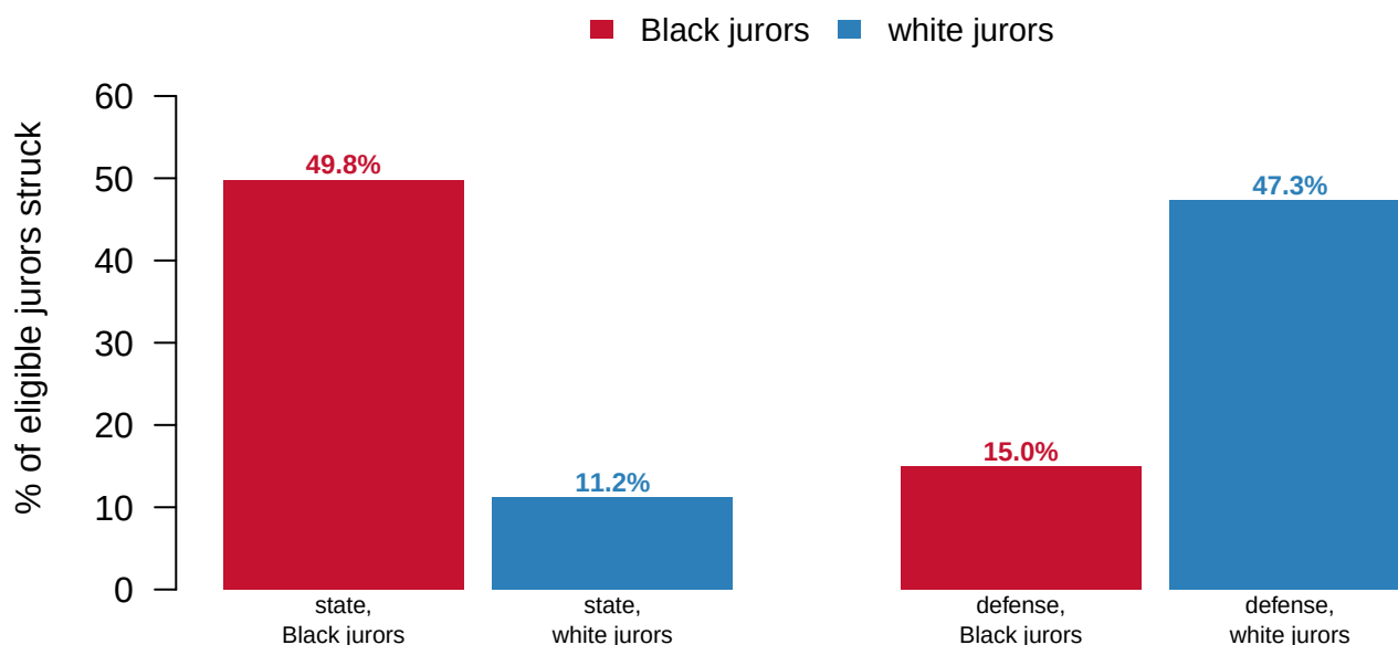
Figure 1. The two sides strike the same panels in opposite directions. Four bars, because the claim is about four rates measured on the same jurors, and a bar makes shares comparable at a glance. Across 211 trials the state struck 49.8% of eligible Black jurors and 11.2% of eligible white ones; the defense struck 47.3% of eligible white jurors and 15.0% of eligible Black ones. The two tall bars differ by 2.5 points and the two short ones by 3.8.
