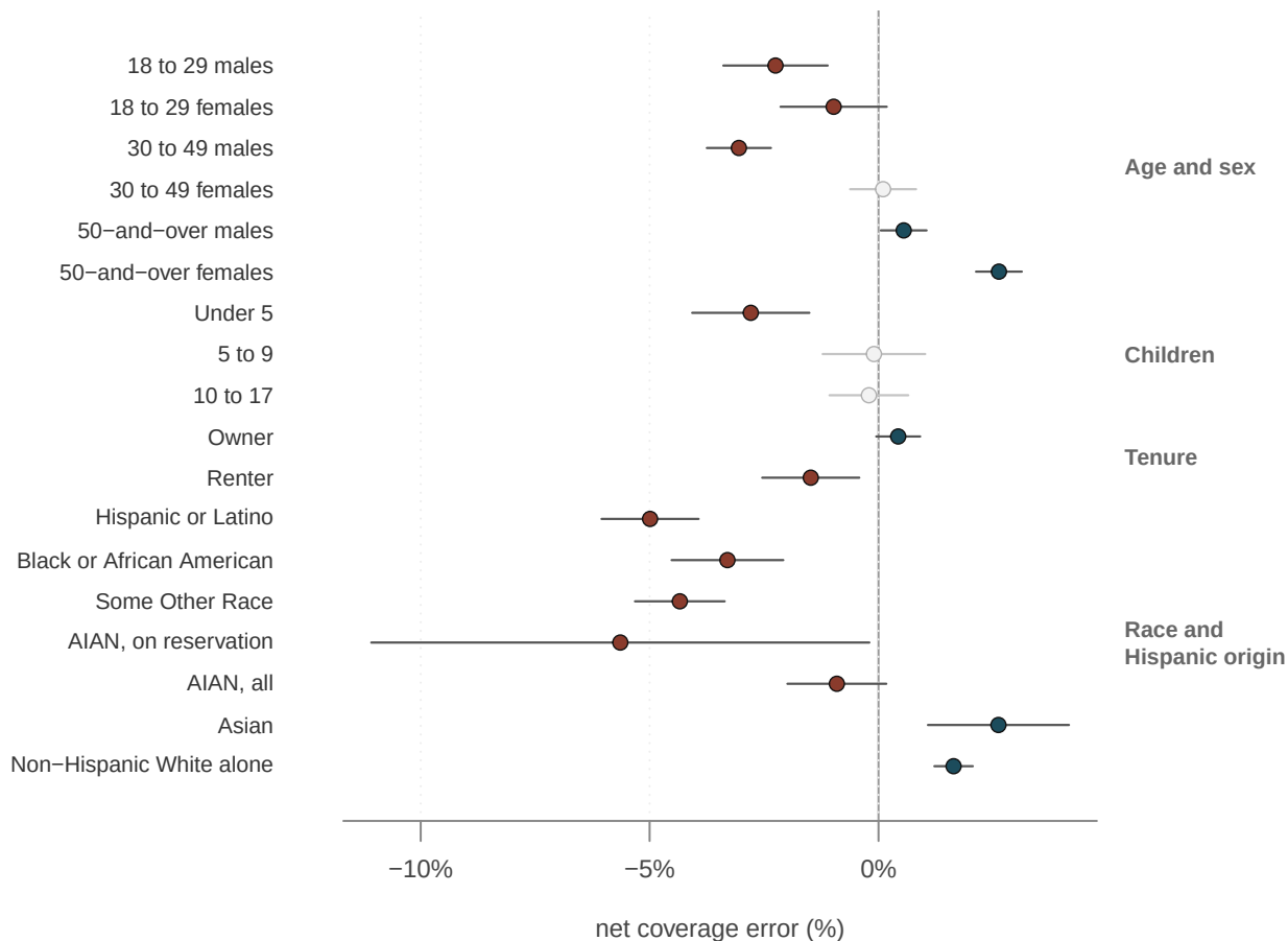
Figure 2. Every national demographic estimate in this brief, with the margin the Bureau prints beside it drawn to scale. Filled circles are rows the Bureau characterizes; hollow circles are rows where it says nothing. The bars are short, a median of 0.48 points here against 1.43 for a state, because a national group is measured with the whole sample while a state gets only its own slice.
