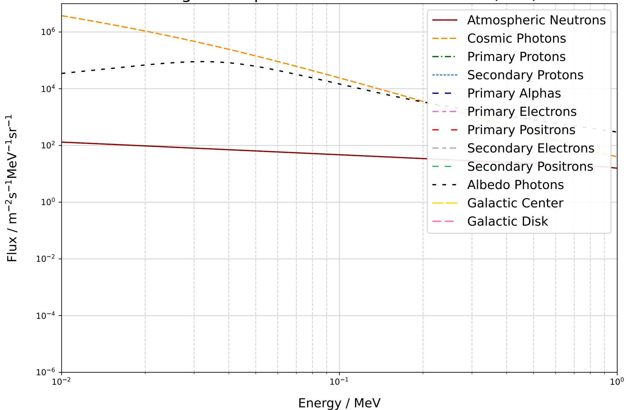
Background spectrum in a low Earth orbit (LEO)
