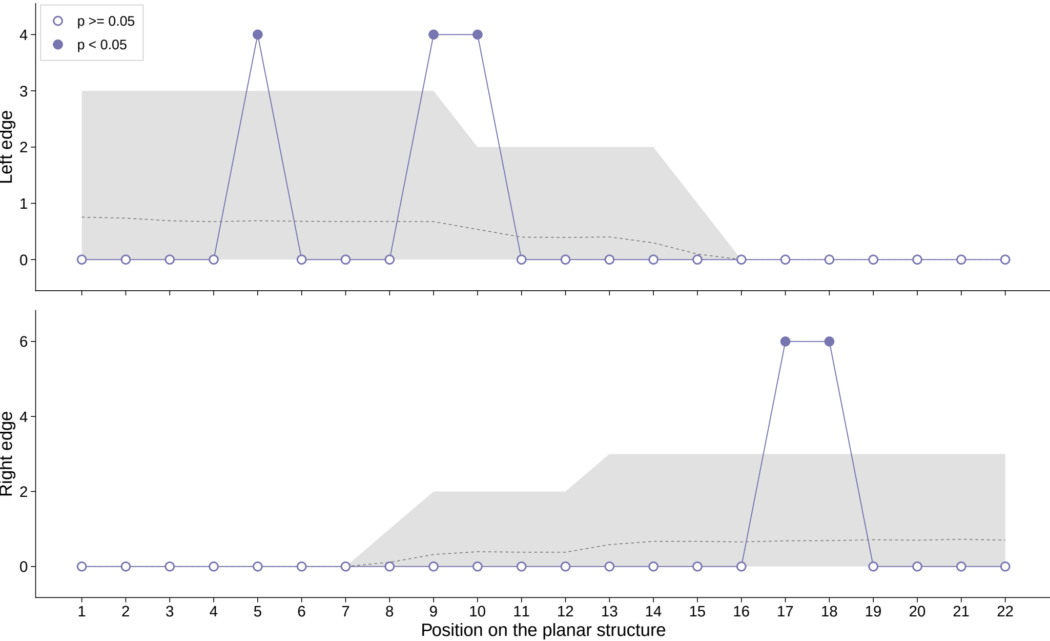
Strength vs. a same-length-profile random null – Length
