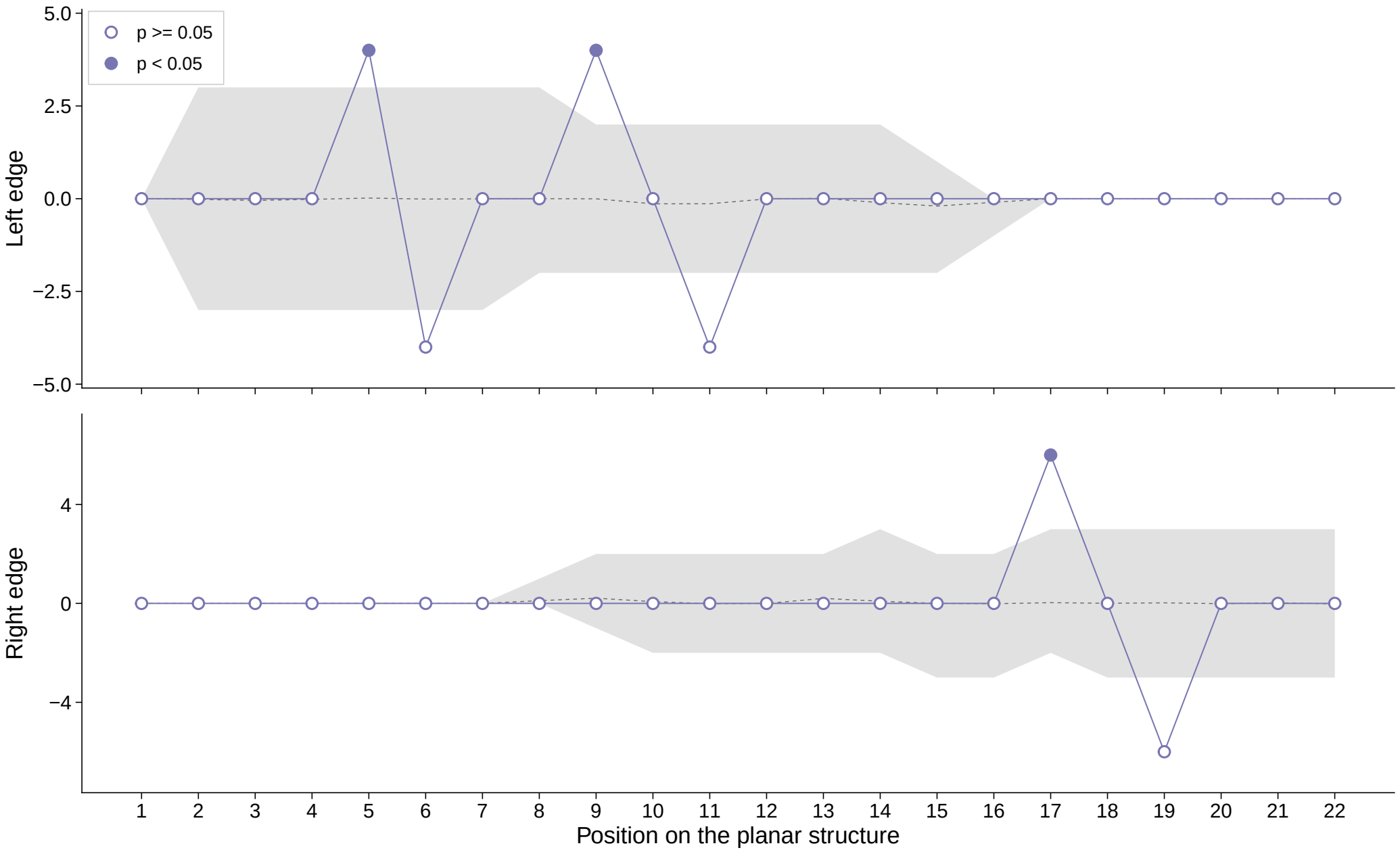
Jump from previous position vs. a same-length-profile random null – Length
