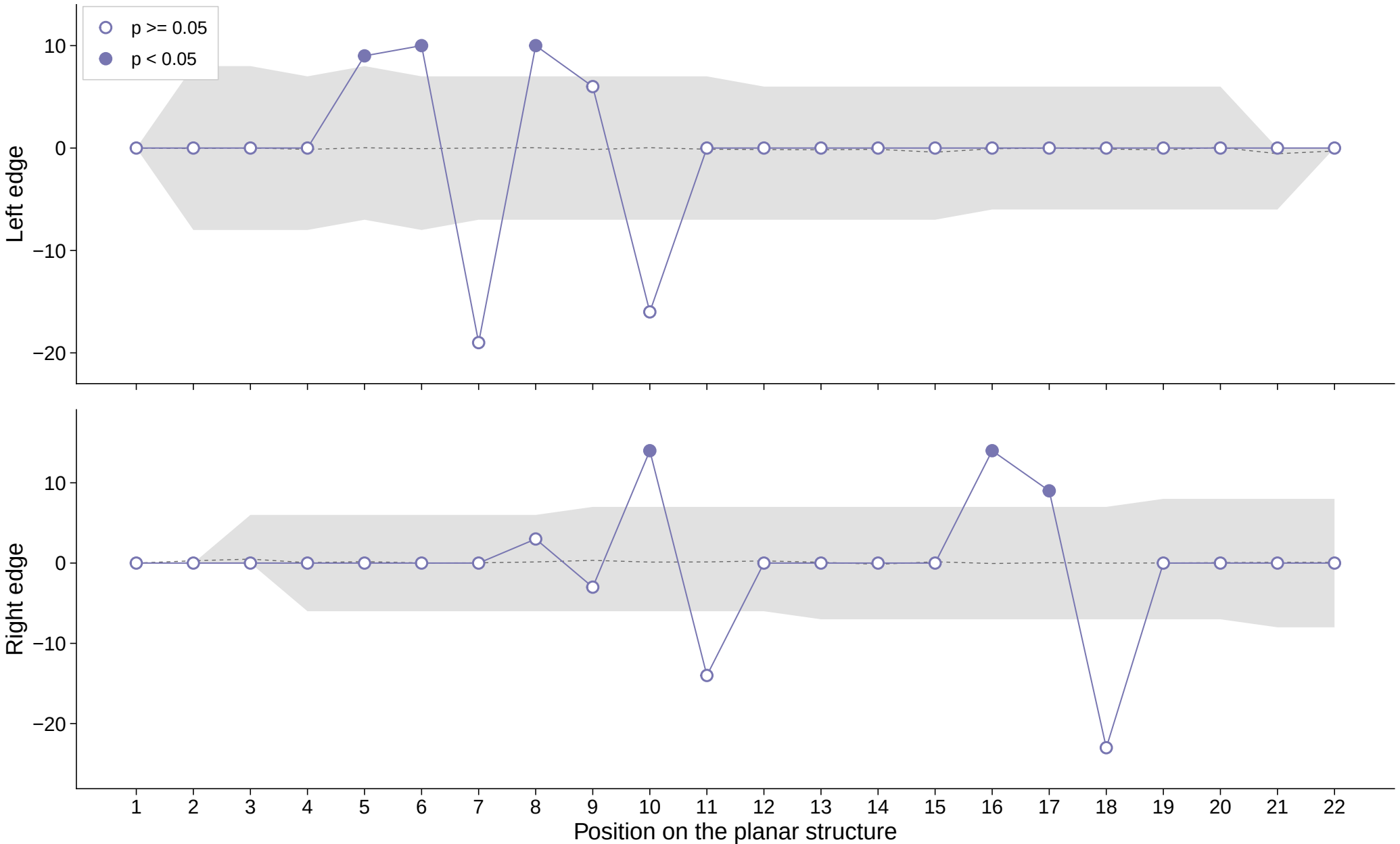
Jump from previous position vs. a same-length-profile random null – Tonosegmental
