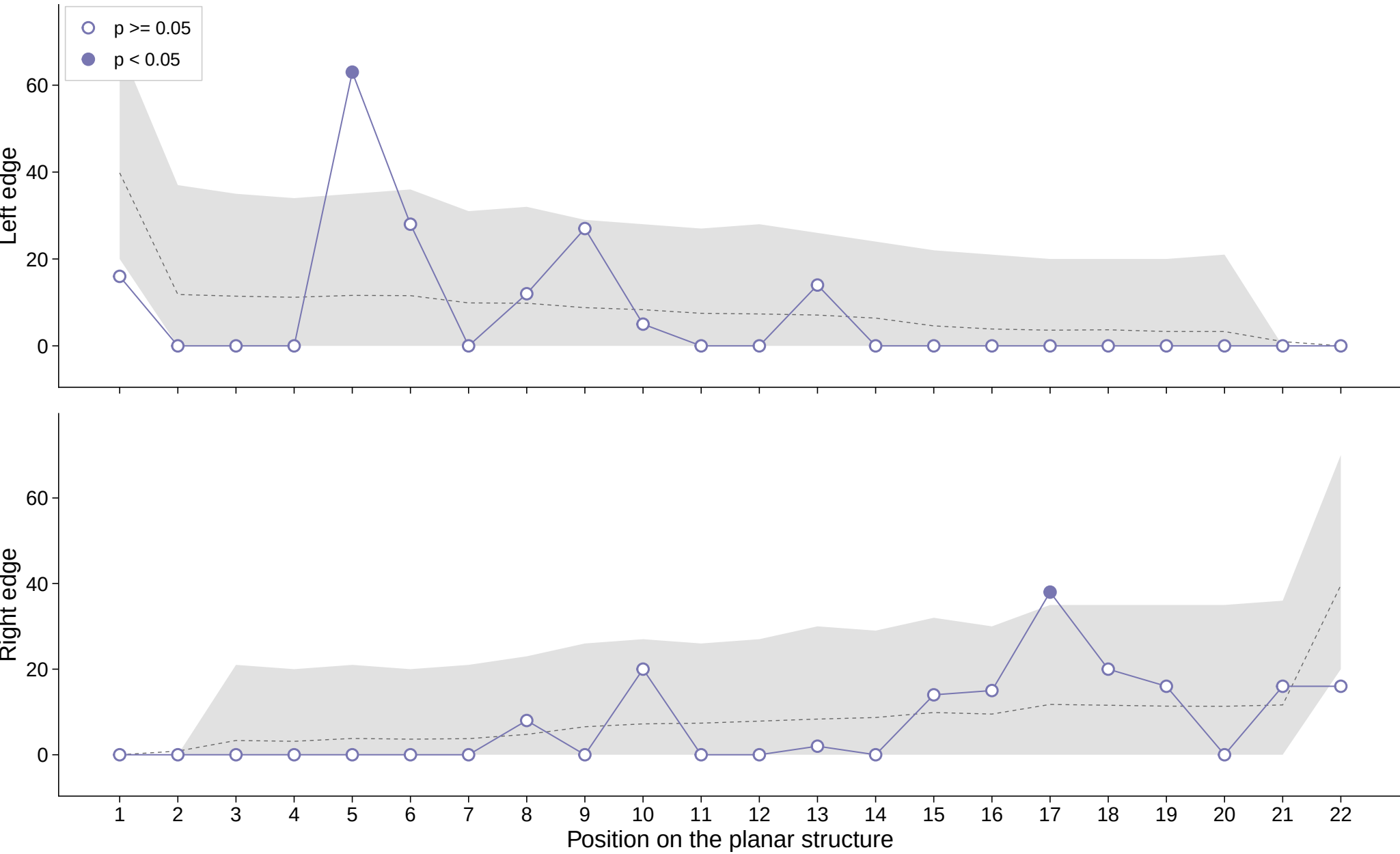
Strength vs. a same-length-profile random null – Syntax-like
