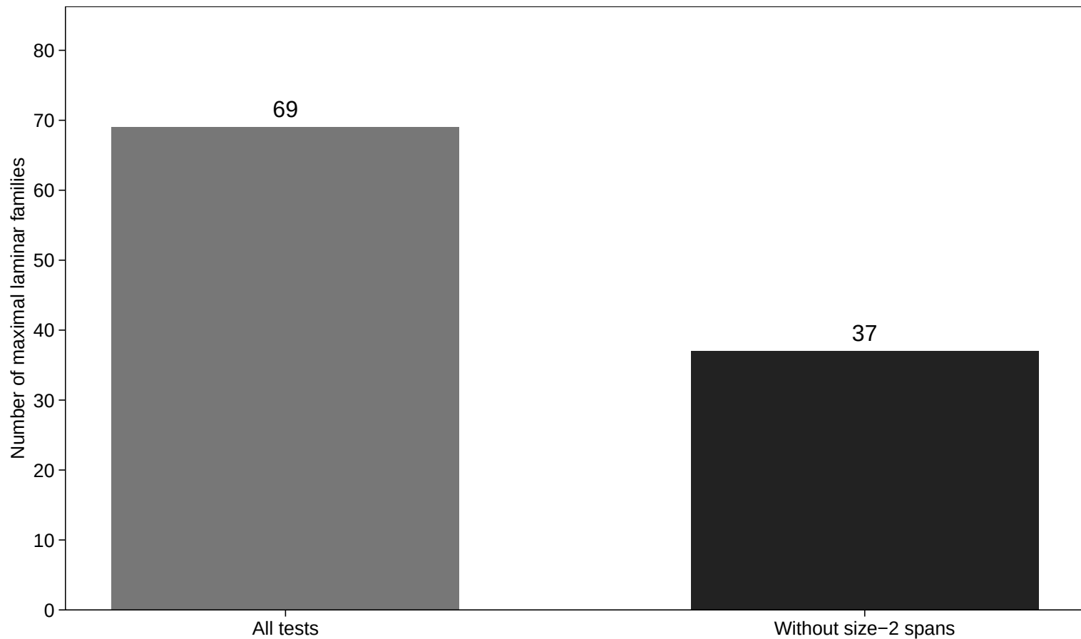
Shifted test data (shifted_nyan): effect of removing adjacent spans
