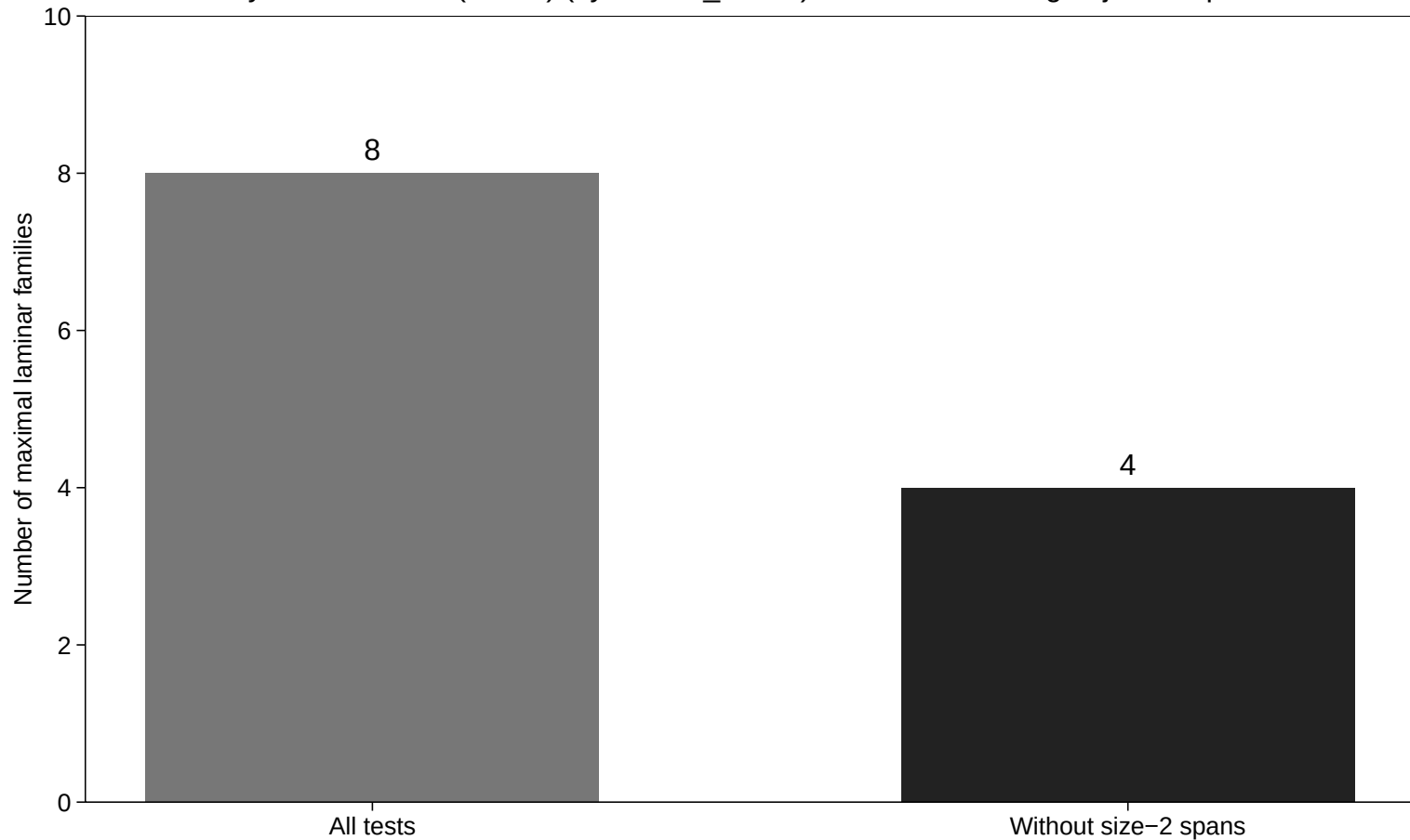
Ayautla Mazatec (verbal) (ayau1235_verbal): effect of removing adjacent spans
