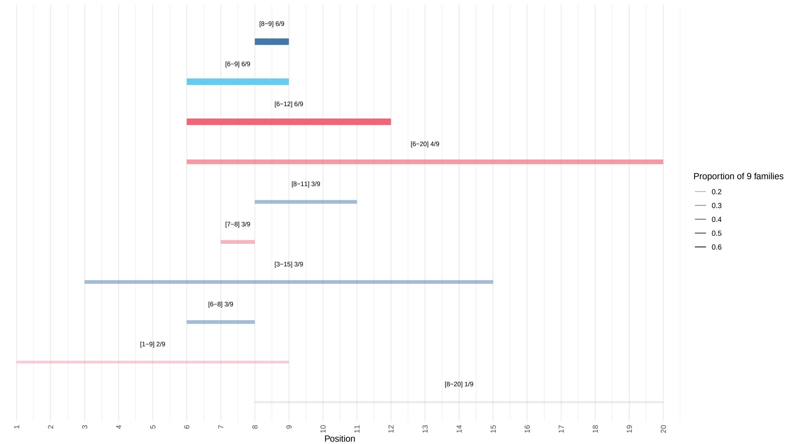
9 maximal families: span frequencies
