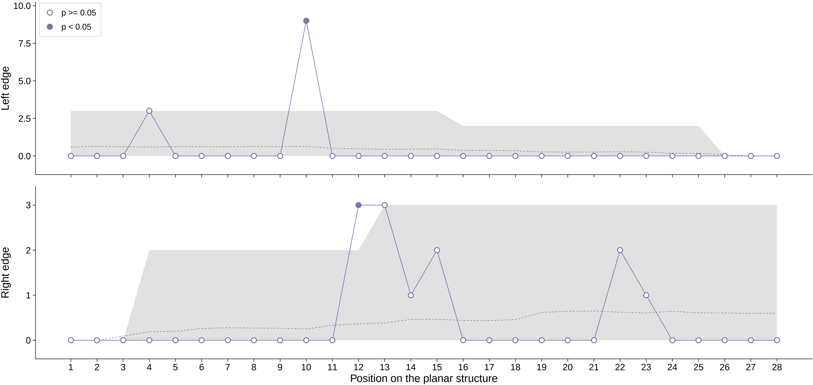
Strength vs. a same-length-profile random null – Morphosyntactic + indeterminate
