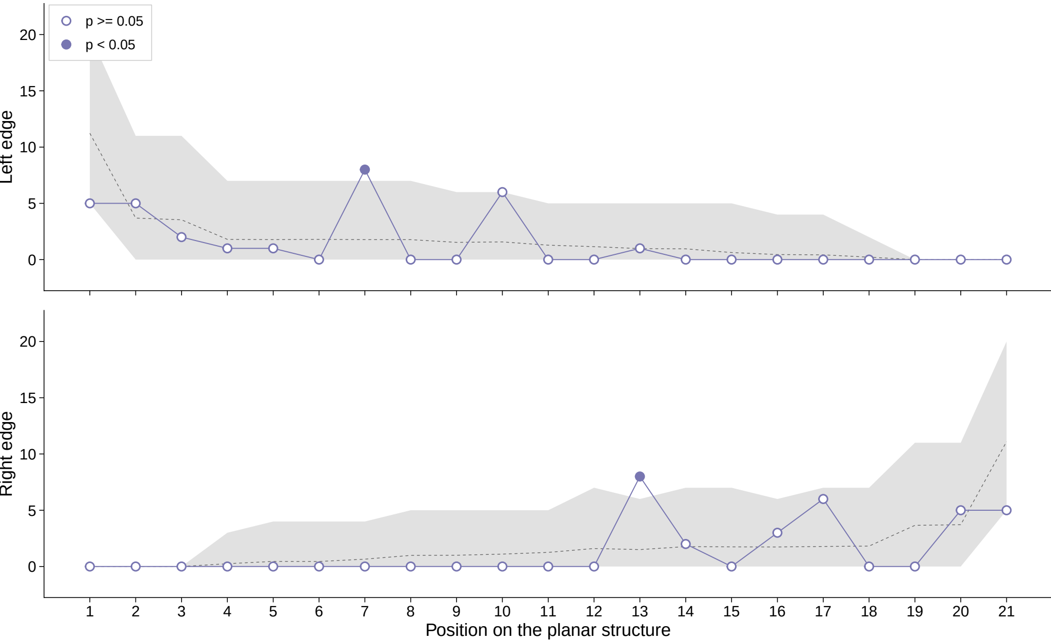
Strength vs. a same-length-profile random null – All tests
