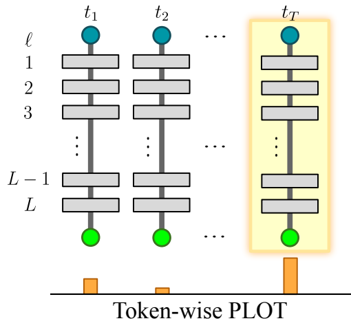
Neural model
