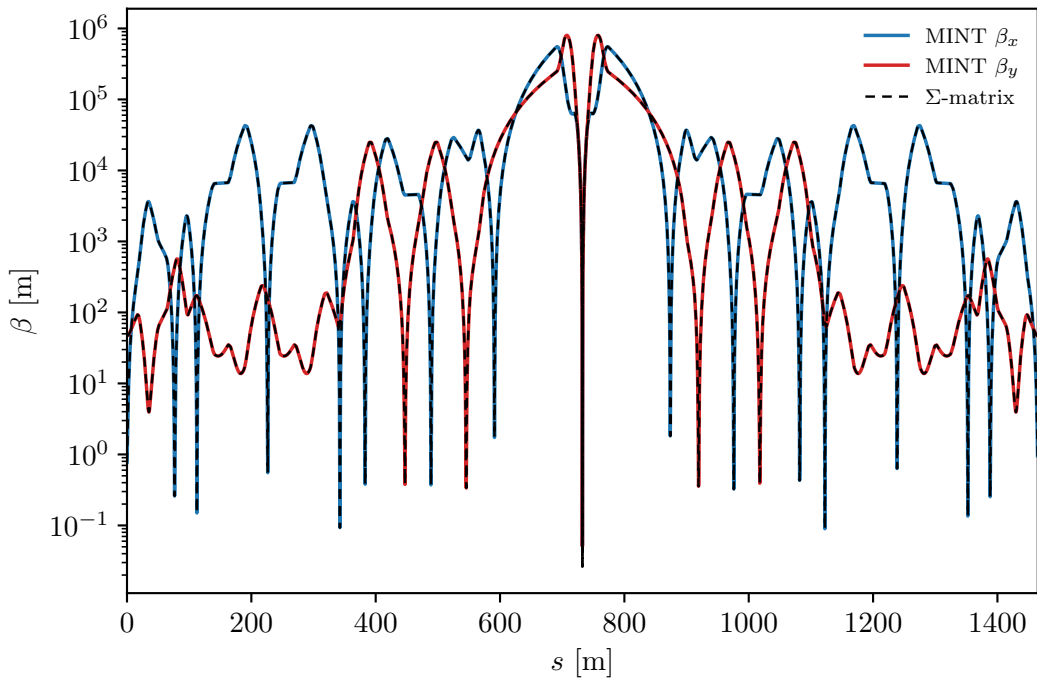
Courant-Snyder \beta function
