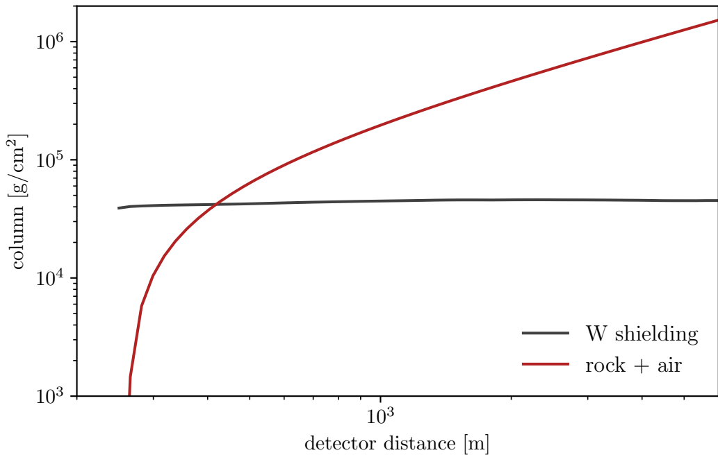
Flux-weighted material in front of the detector
