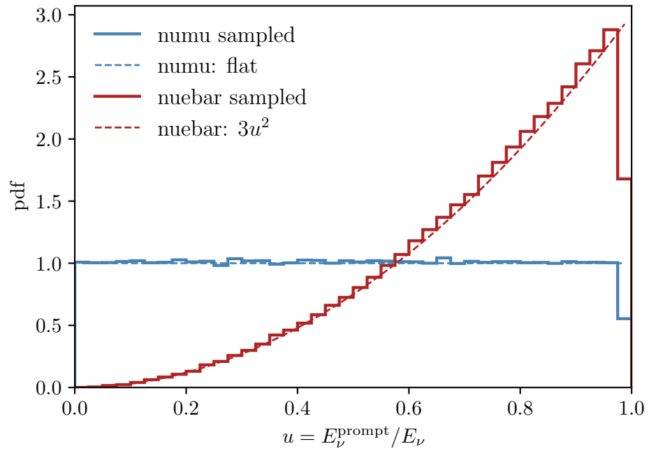
IMD at 1 TeV
