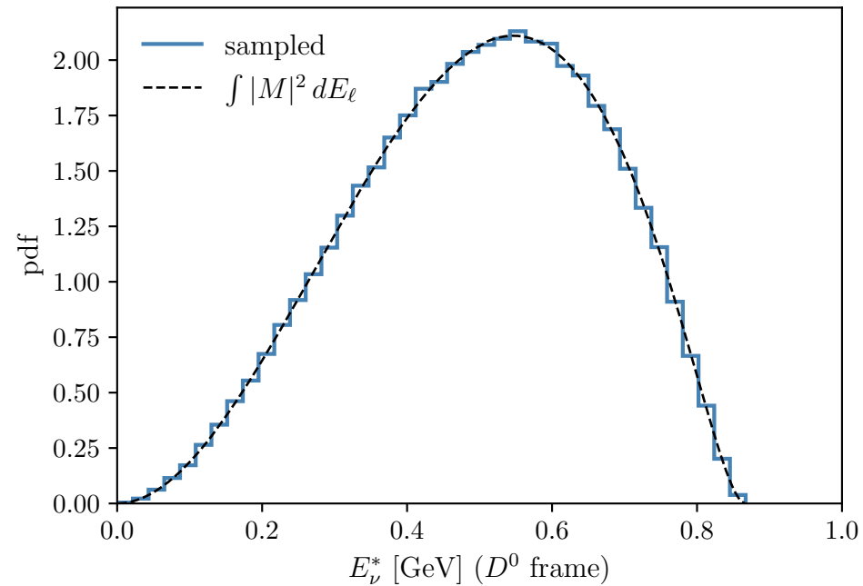
D \rightarrow K \ell \nu Dalitz
