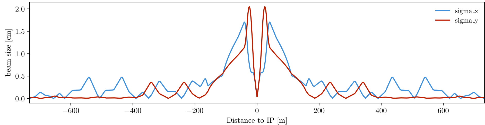
Beam envelope (RMS)
