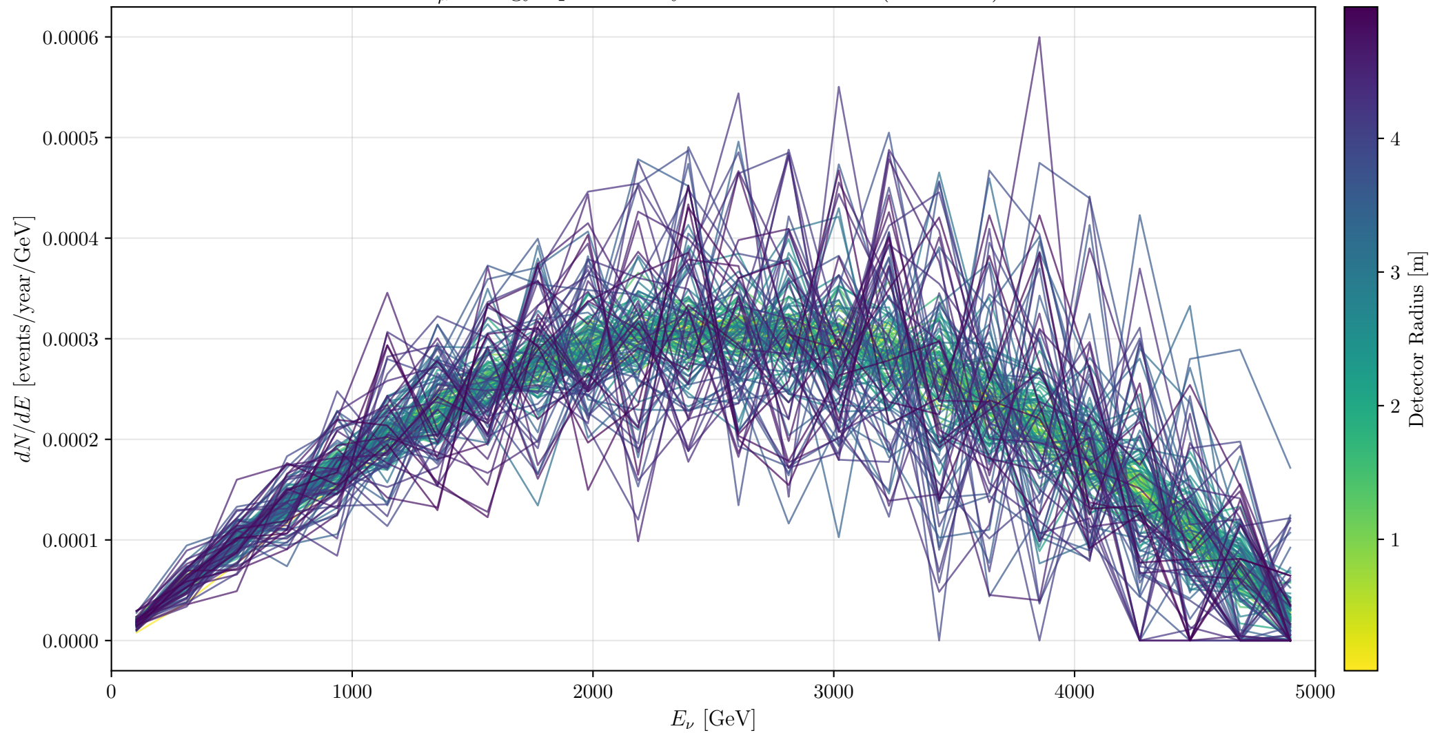
\bar{\nu}_\mu Energy Spectrum by Detector Radius ( z = 1 km)
