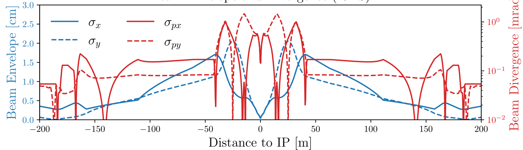
Beam Envelope and Divergence (RMS)
