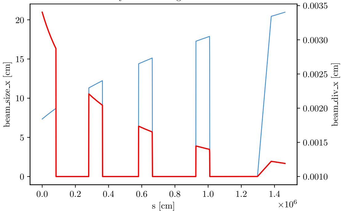
Beam Dynamics Along RLA2 Lattice
