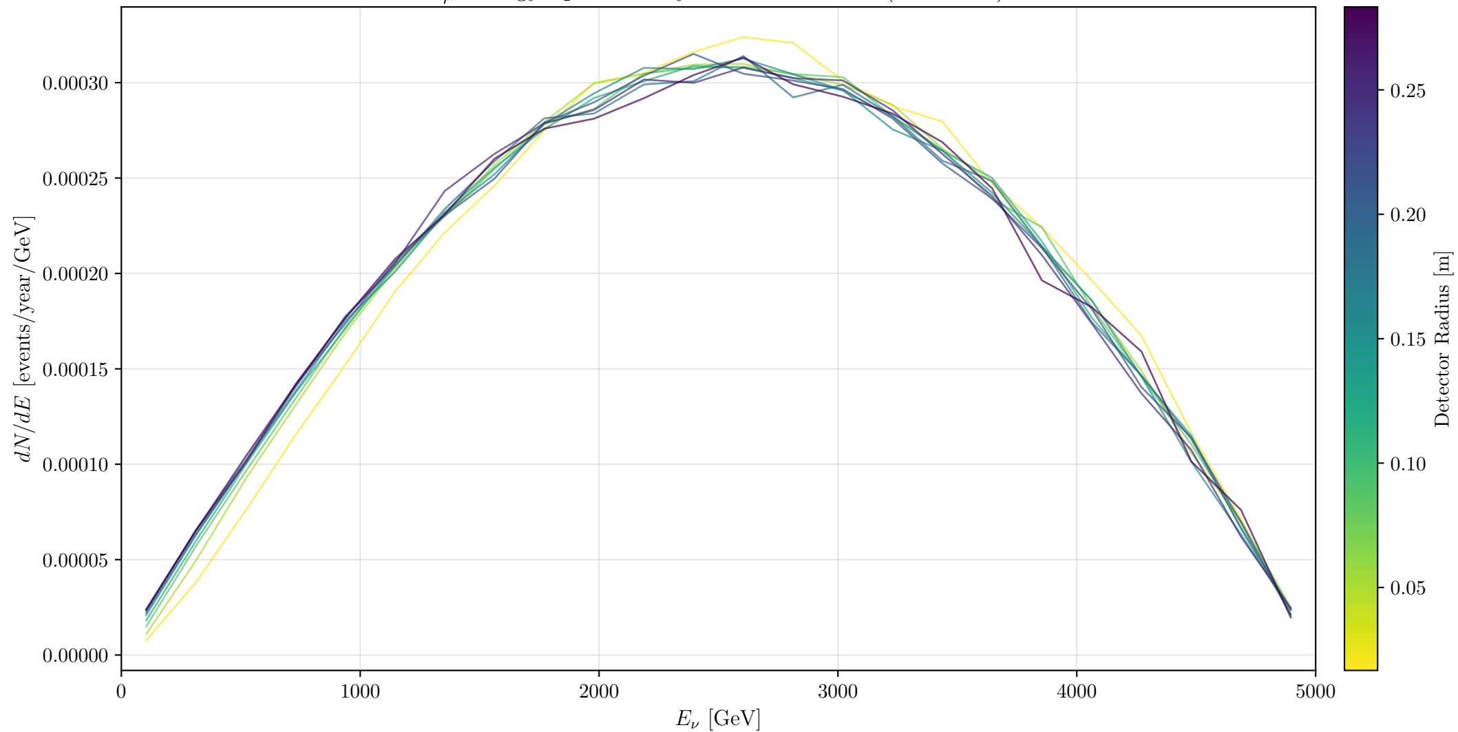
\bar{\nu}_\mu Energy Spectrum by Detector Radius ( z = 1 km)
