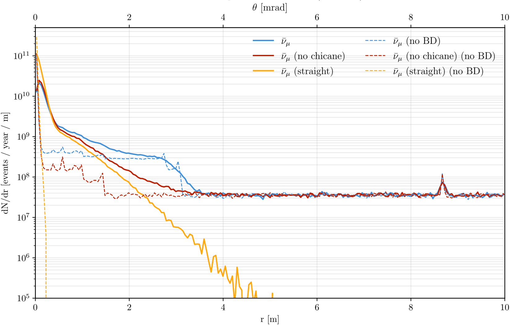
Event Rate per Detector Radius ( z = 1 km)
