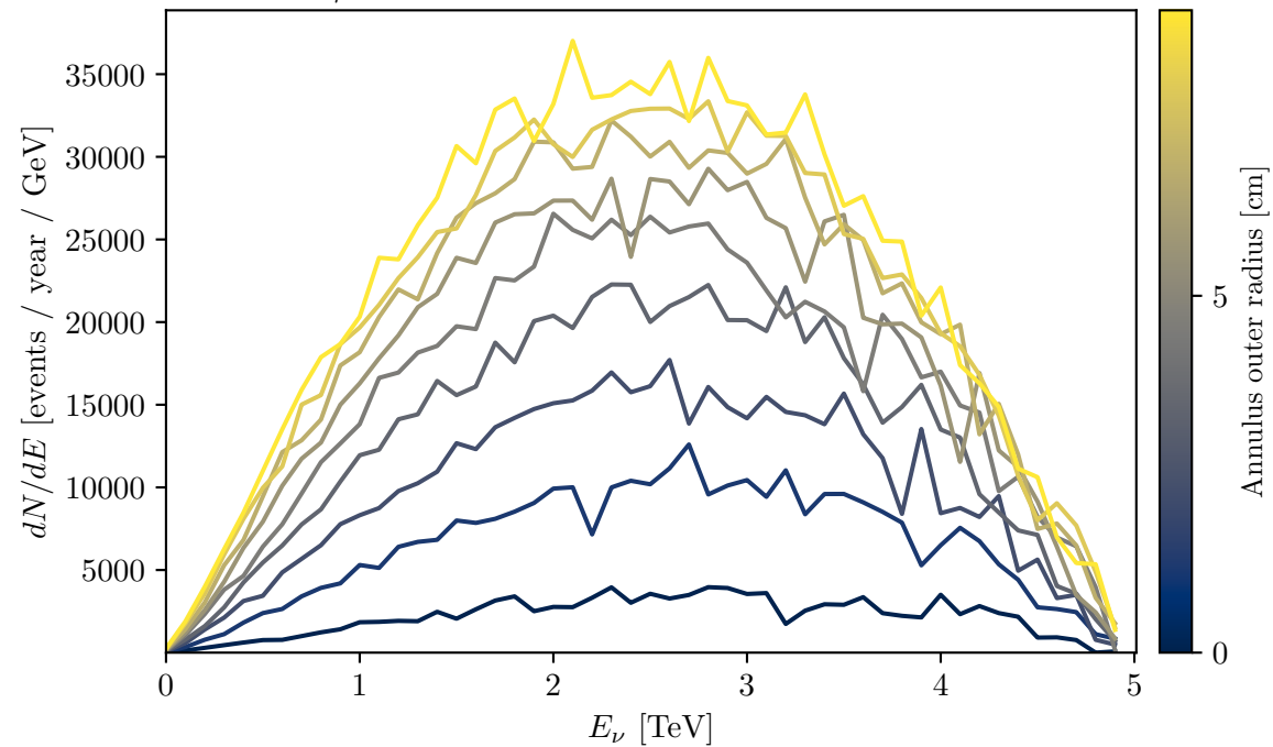
\bar{\nu}_\mu annular spectrum, L = 1 km, \ell_{\text{det}} = 10 m
