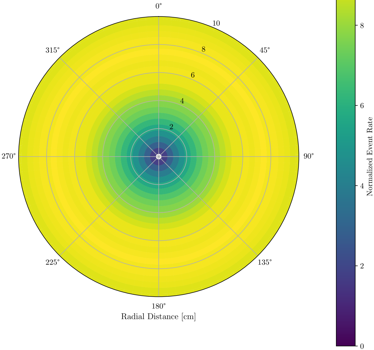
\bar{\nu}_\mu Event Rate by Detector Radius
