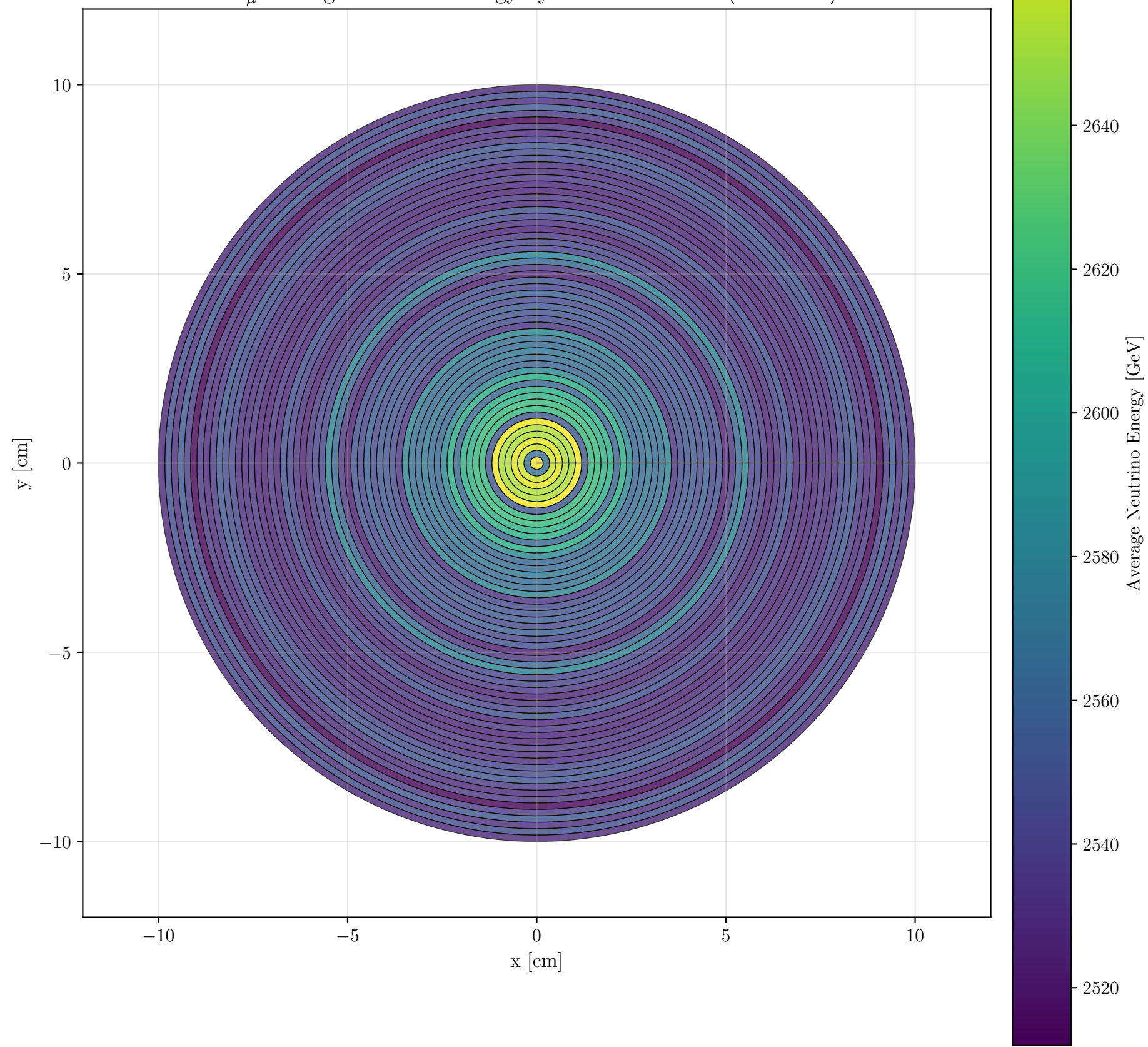
\bar{\nu}_\mu Average Neutrino Energy by Detector Radius ( z = 1 km)
