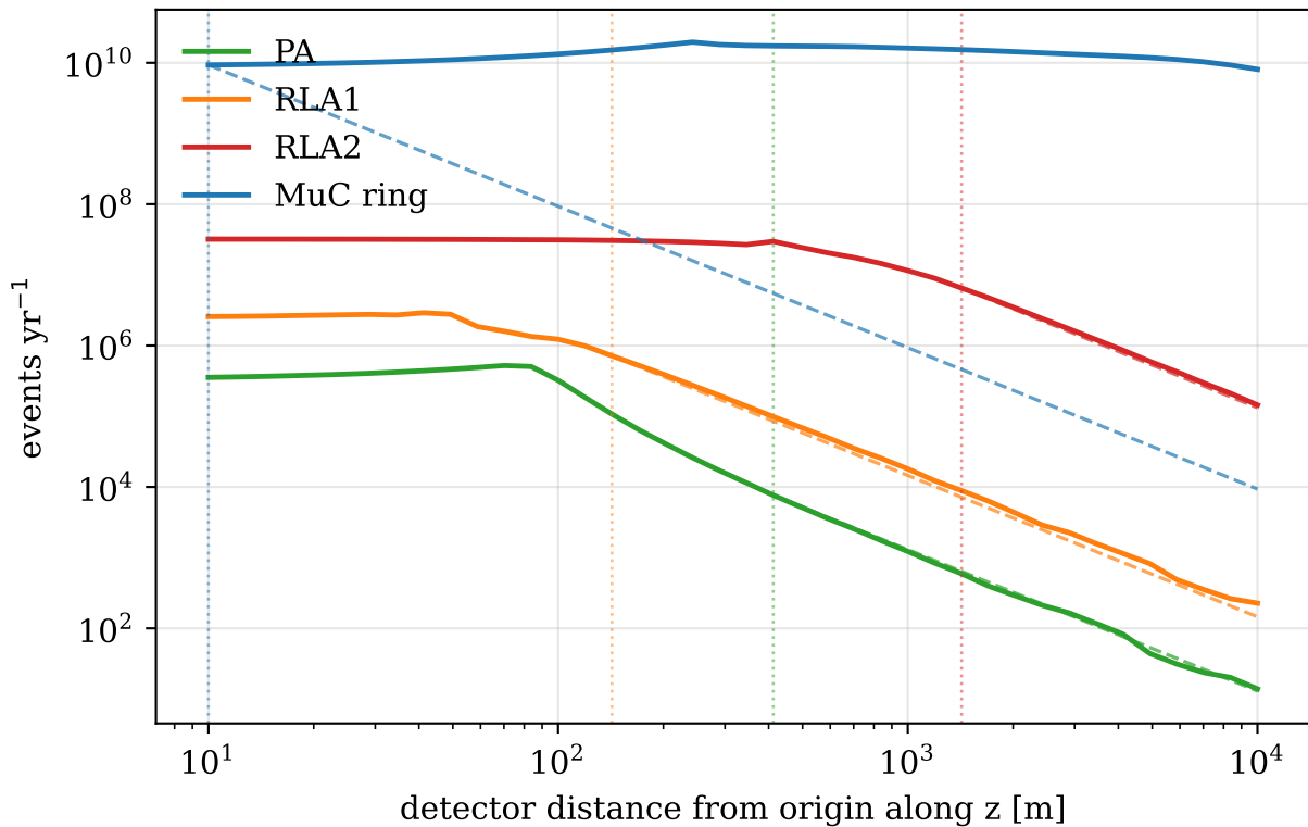
Benchmark-detector event counts vs. z (numubar)
