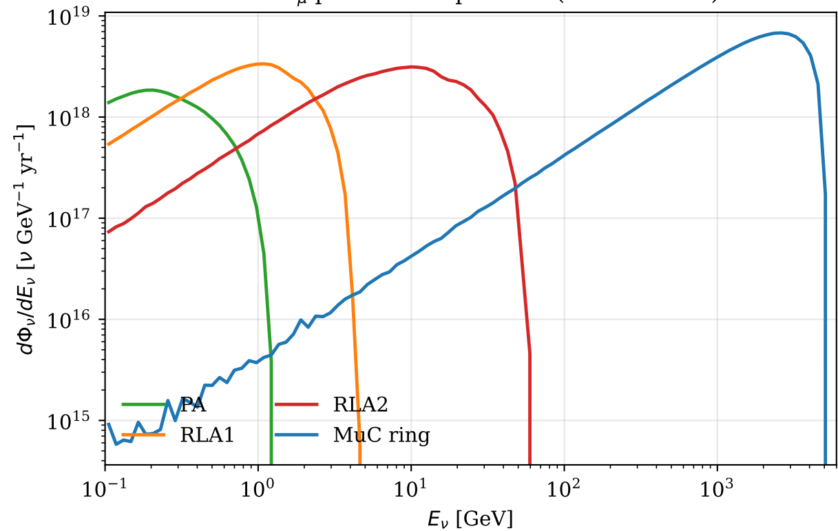
Total \bar{\nu}_\mu production spectrum (all directions)
