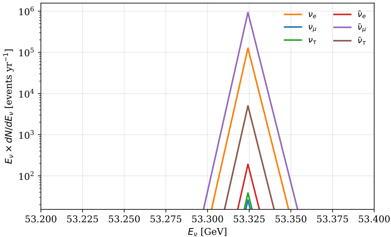
RLA2 oscillated events at L = 1300 km, r < 2 km
