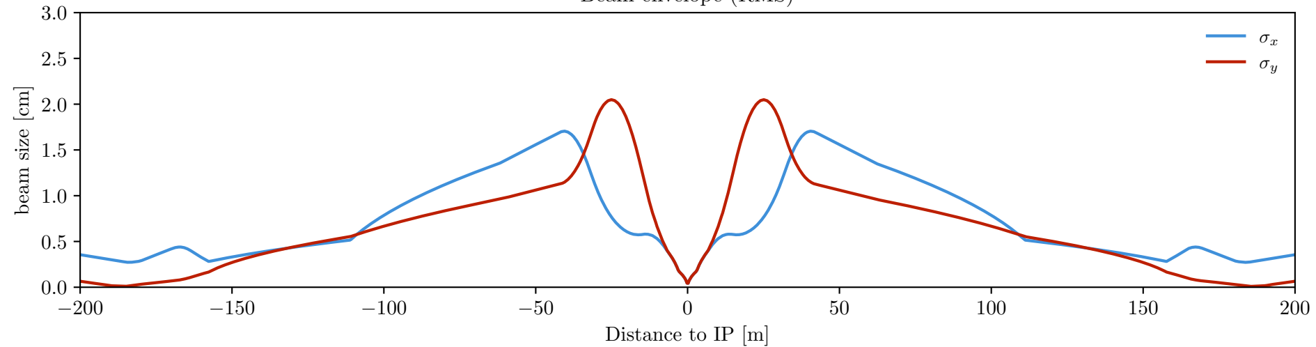
Beam envelope (RMS)
