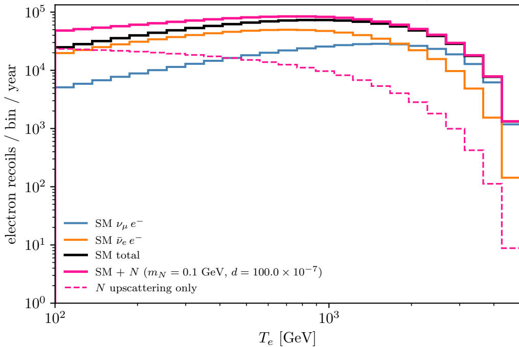
\nu e^- scattering at the HPGAr detector ( \mu^- beam), 10 yr
