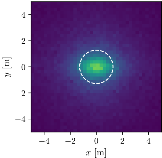
\mu^+ beam ( z = 5 km)
