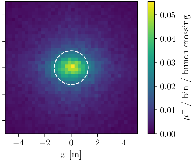
\mu^- beam ( z = -5 km)
