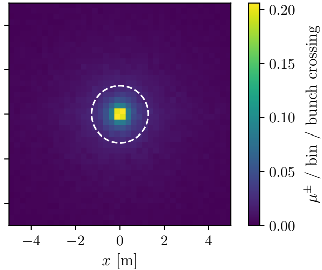
\mu^- beam, beam dyn. off
