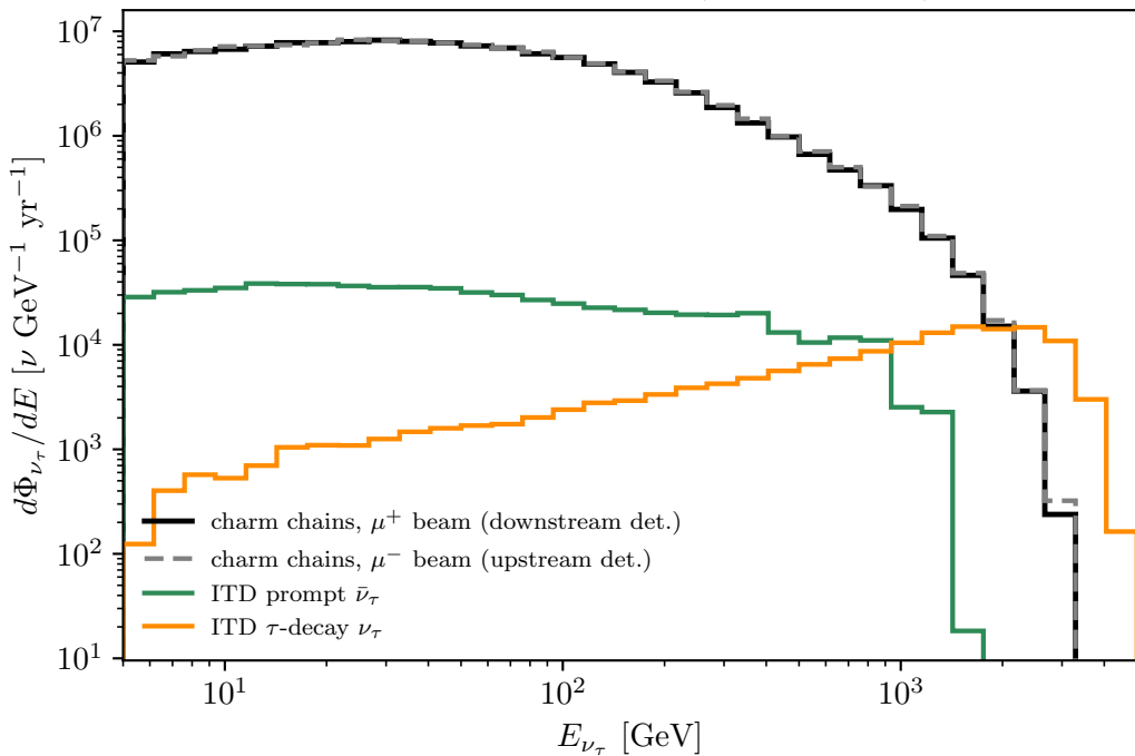
Secondary \nu_\tau : all sources (MC kinematics)
