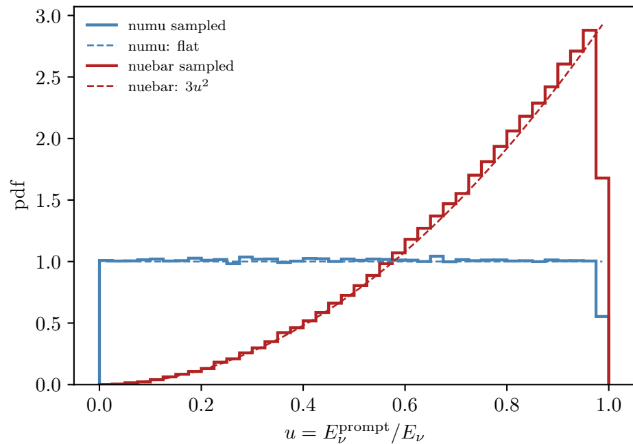
IMD prompt-neutrino spectrum at 1 TeV
