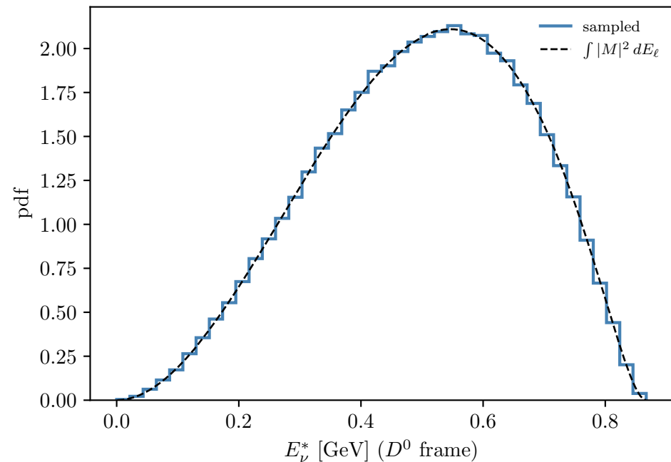
D \rightarrow K\ell\nu : Dalitz sampler vs analytic
