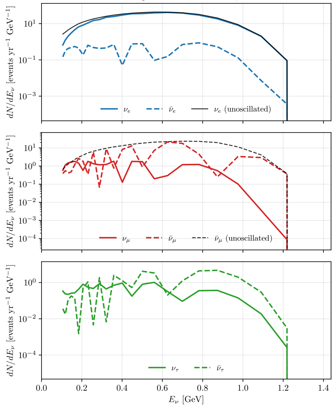
PA oscillated spectra at L = 1300 km, r < 105.0 m
