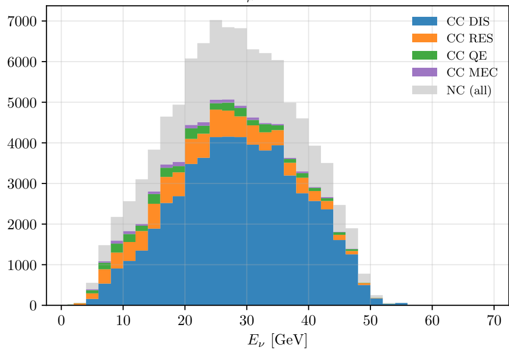
\bar{\nu}_\mu on Ar40
