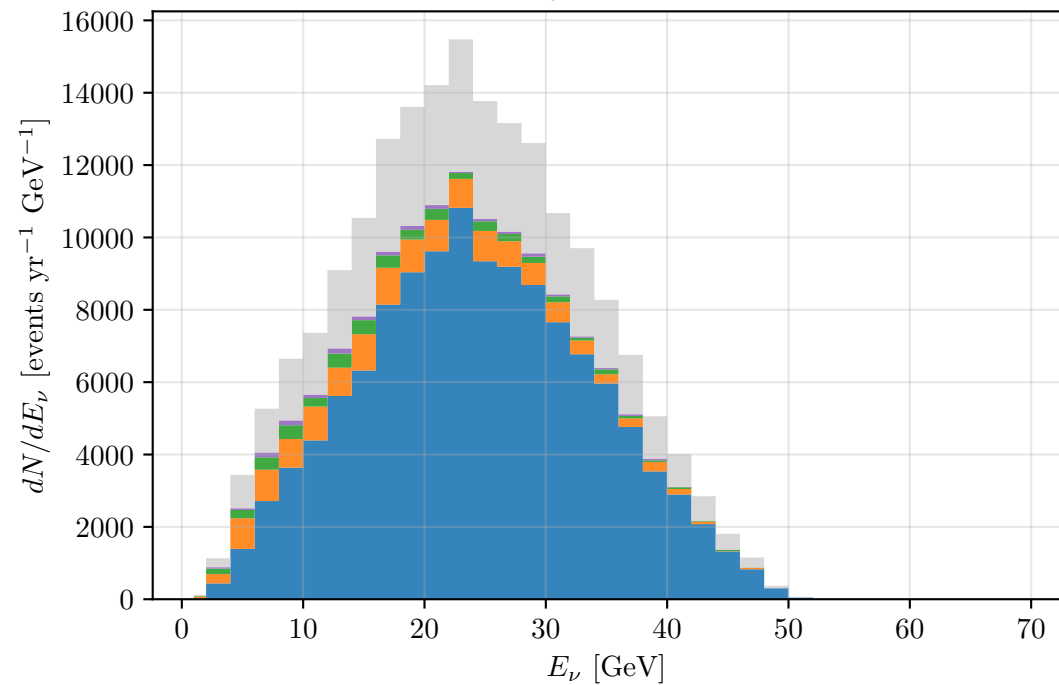
\nu_e on Ar40
