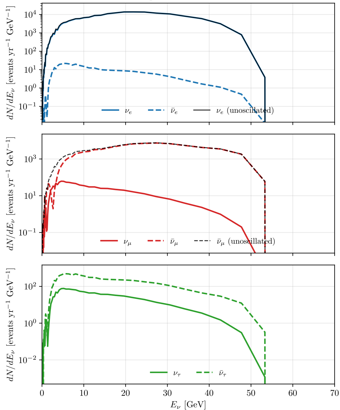
RLA2 oscillated spectra at L = 1300 km, r < 105.0 m
