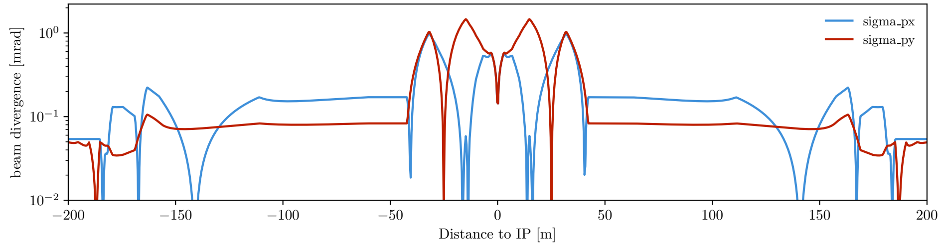
Beam divergence (RMS)
