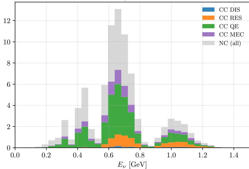
PA: \bar{\nu}_\mu on Ar40
