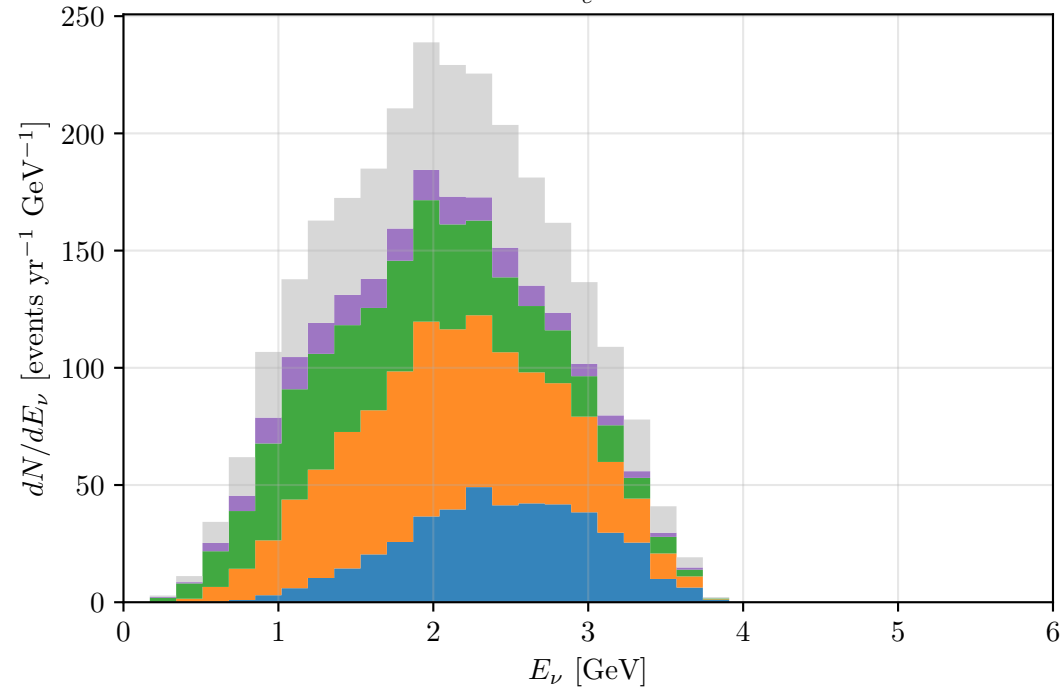
RLA1: \nu_e on Ar40
