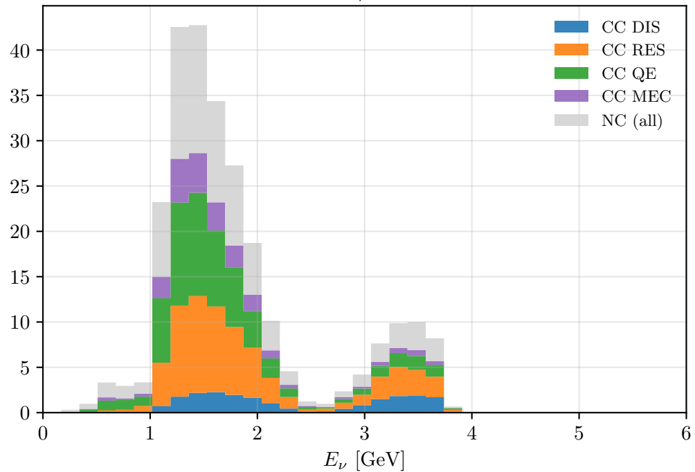
RLA1: \bar{\nu}_\mu on Ar40
