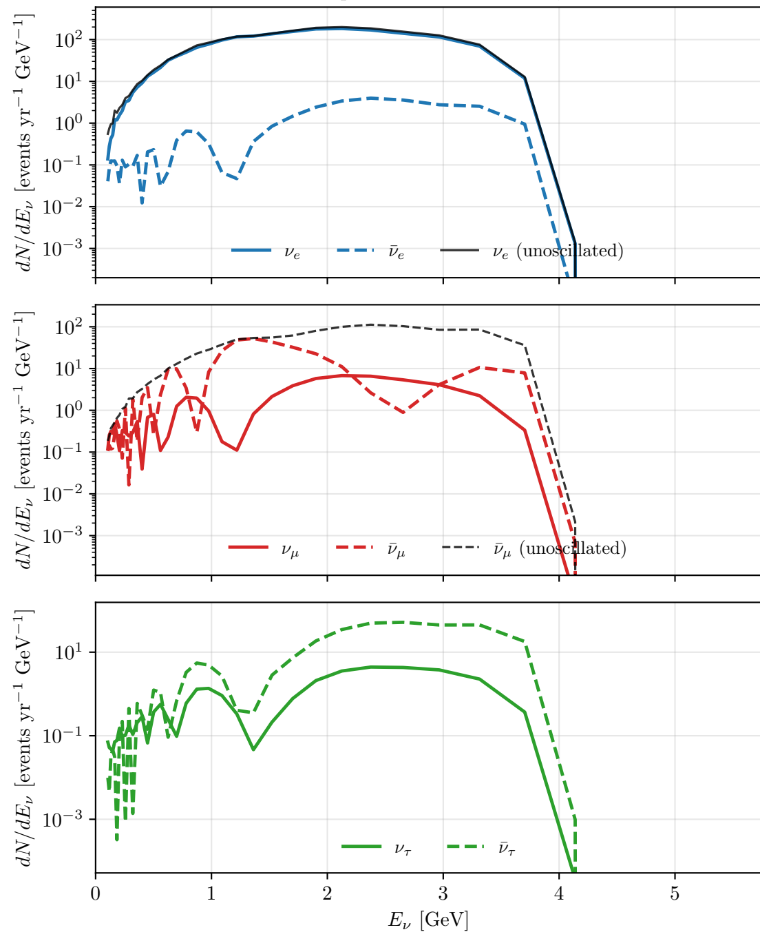
RLA1 oscillated spectra at L = 1300 km, r < 105.0 m
