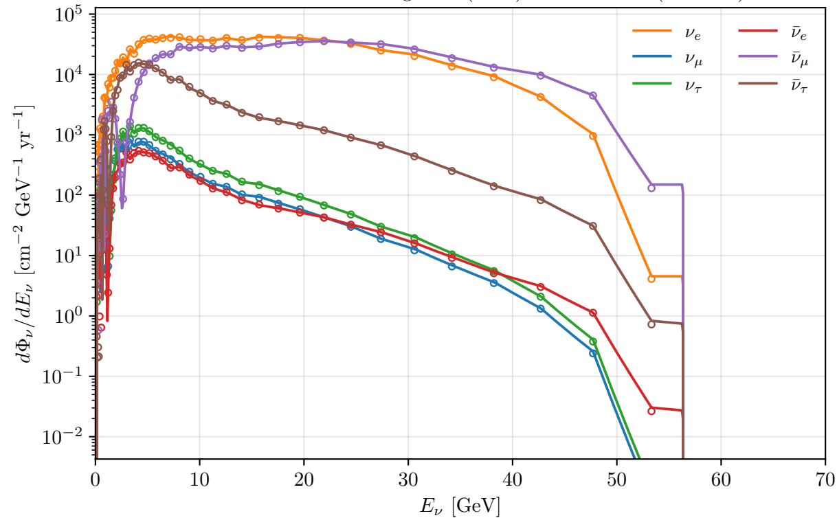
RLA2 GENIE flux histograms (lines) vs. section 8 (markers)
