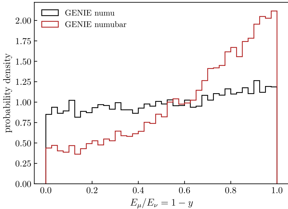
CC muon energy fraction at E_\nu = 600 GeV
