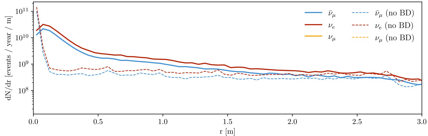
Detector at z = 1 km
