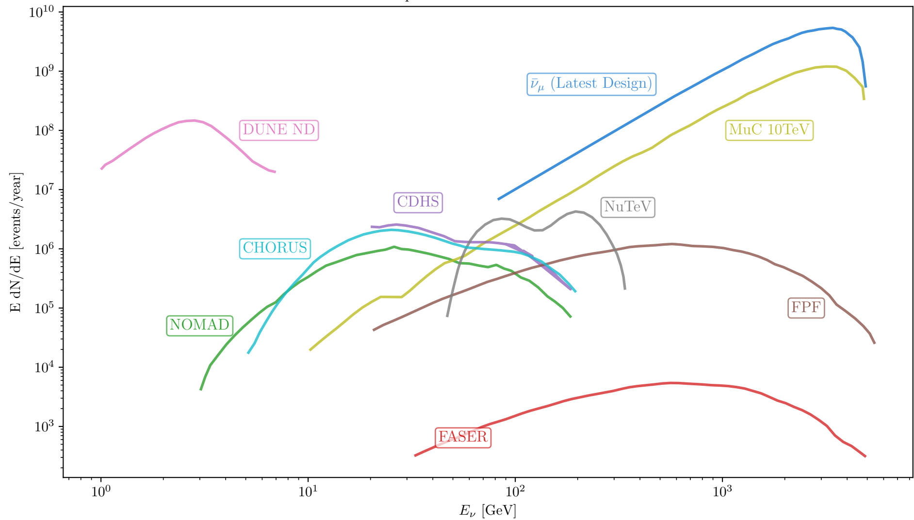
Neutrino Spectrum for a Detector at z = 1 km
