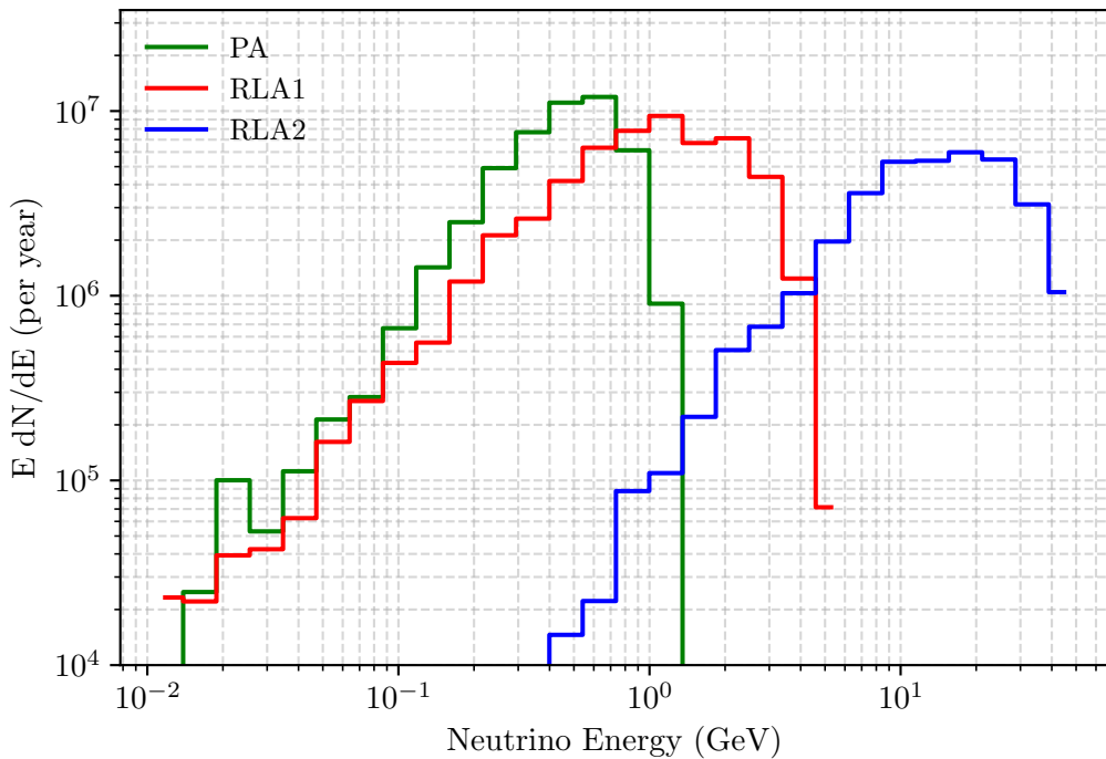
Time Integrated Event Rate at Each Accelerator Complex (with "realistic" detector placement)
