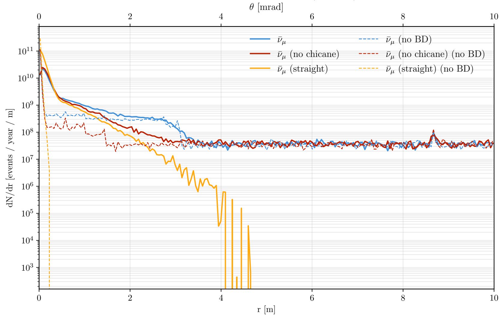
Event Rate per Detector Radius ( z = 1 km)
