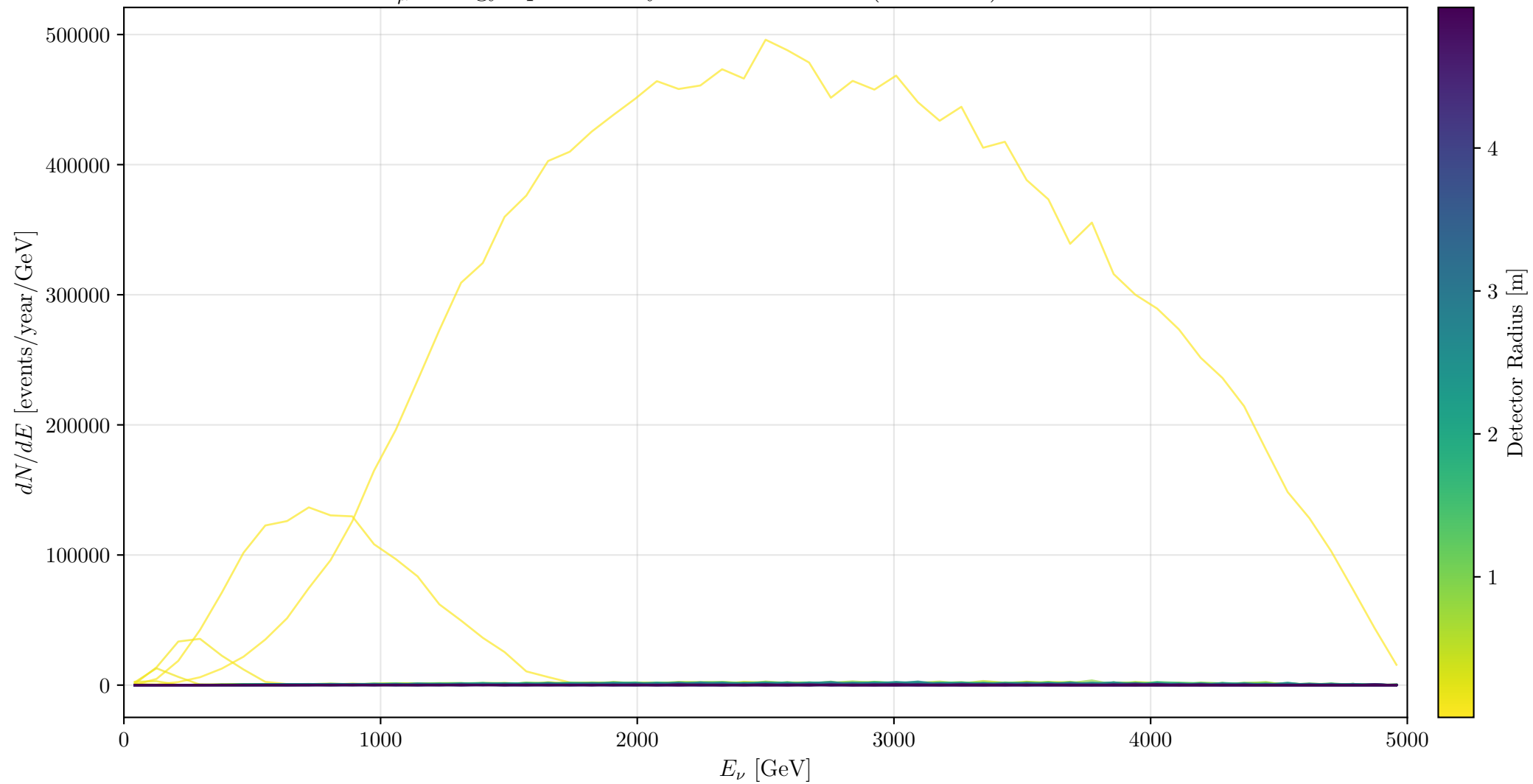
\bar{\nu}_\mu Energy Spectrum by Detector Radius ( z = 1 km) with no BD
