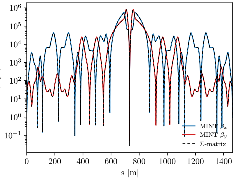
Courant–Snyder \beta function
