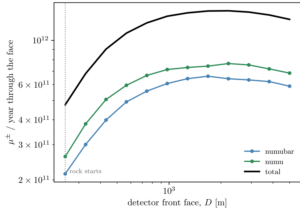
Secondary muons vs detector location
